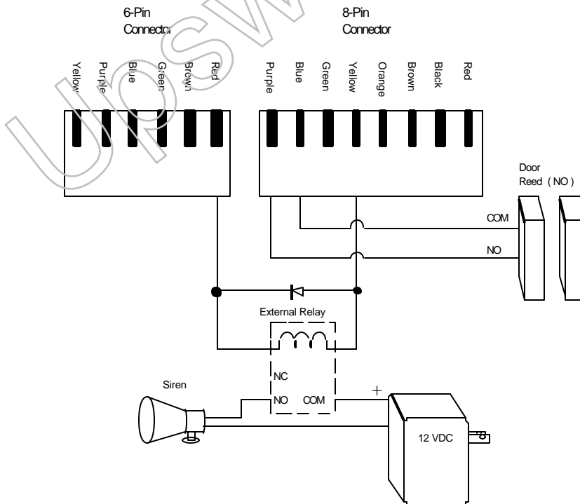
B. Installation of reed switch (normal open), external relay (duress)
