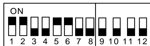
Radio Receiver #2 Right (Upper) Button On Transmitter Controls This Radio
